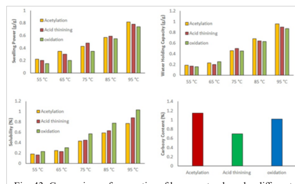
Fig. 43. Comparison of properties of banana starch under different chemical processes
