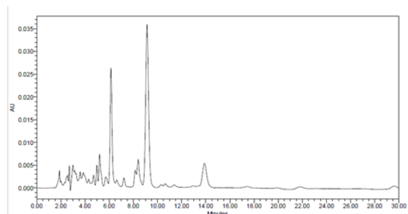
Fig. 48. Chromatogram of major flavonoid compounds in peel of ripe fruit of cv. Monthan; Peak with R_t of 6.0 min is epicatechin; peak with R_t of 9.1 min is galliccatechin and peak with R_t of 13.8 min is catechin
